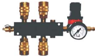
Multi-Pump - For up to 4 pumps - With regulator - Requires 1 pump adapter per pump P/N BGA-MSC-01
